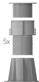
T-Pillar-220 + 5xT-Pillar-CL-140
